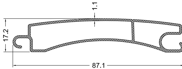
9307-11 0.667 Kg/m
