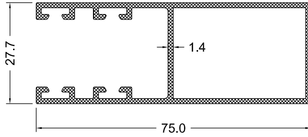
9311 0.910 Kg/m
