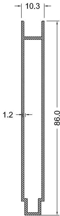
LM 1077-20 1.488 Kg/m
