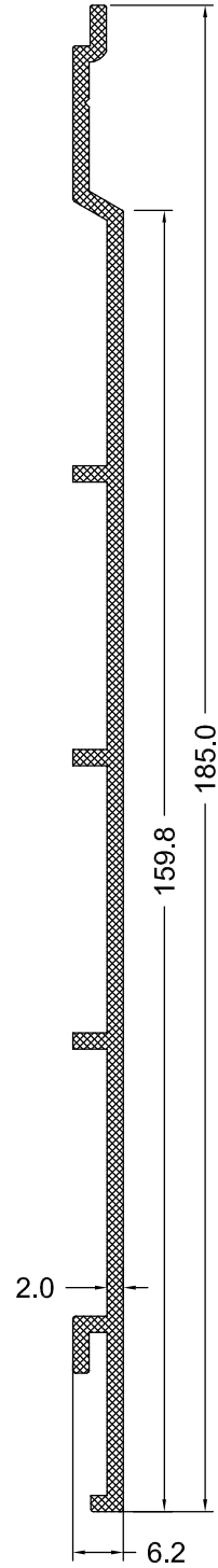
LM 13-20 1.152 Kg/m
