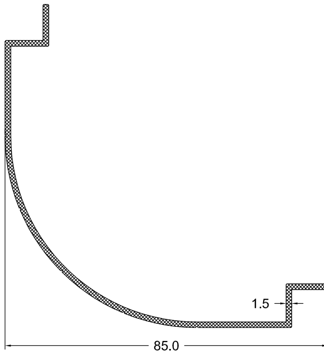
LM 51-15 0.678 Kg/m
