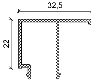
WT 41-13 0.318 Kg/m
