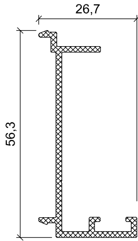
WT 51-16 0.455 Kg/m
