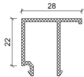
WT 42-15 0.342 Kg/m
