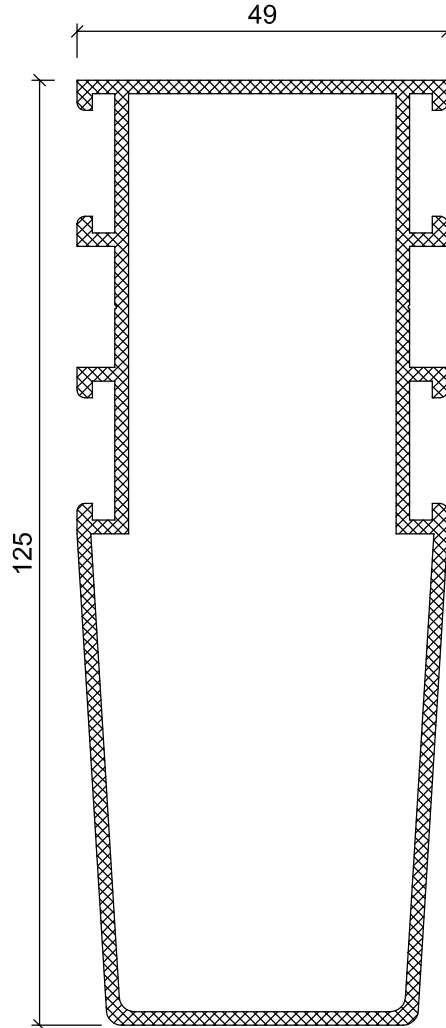
WT 17-18 1.862 Kg/m
