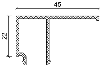
WT 40-15 0.410 Kg/m
