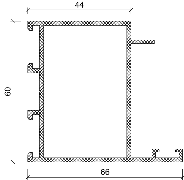
WT 31-18 1.260 Kg/m
